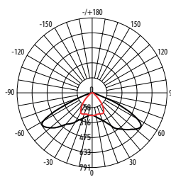
PSL 02 100W 5000K IP65
